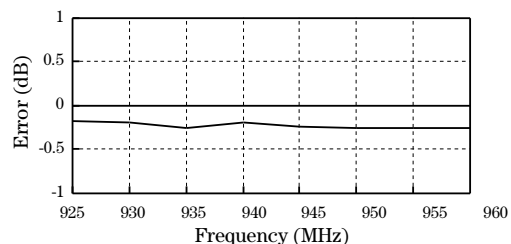
Typical RF generator RF in/out level error at -104 dBm
