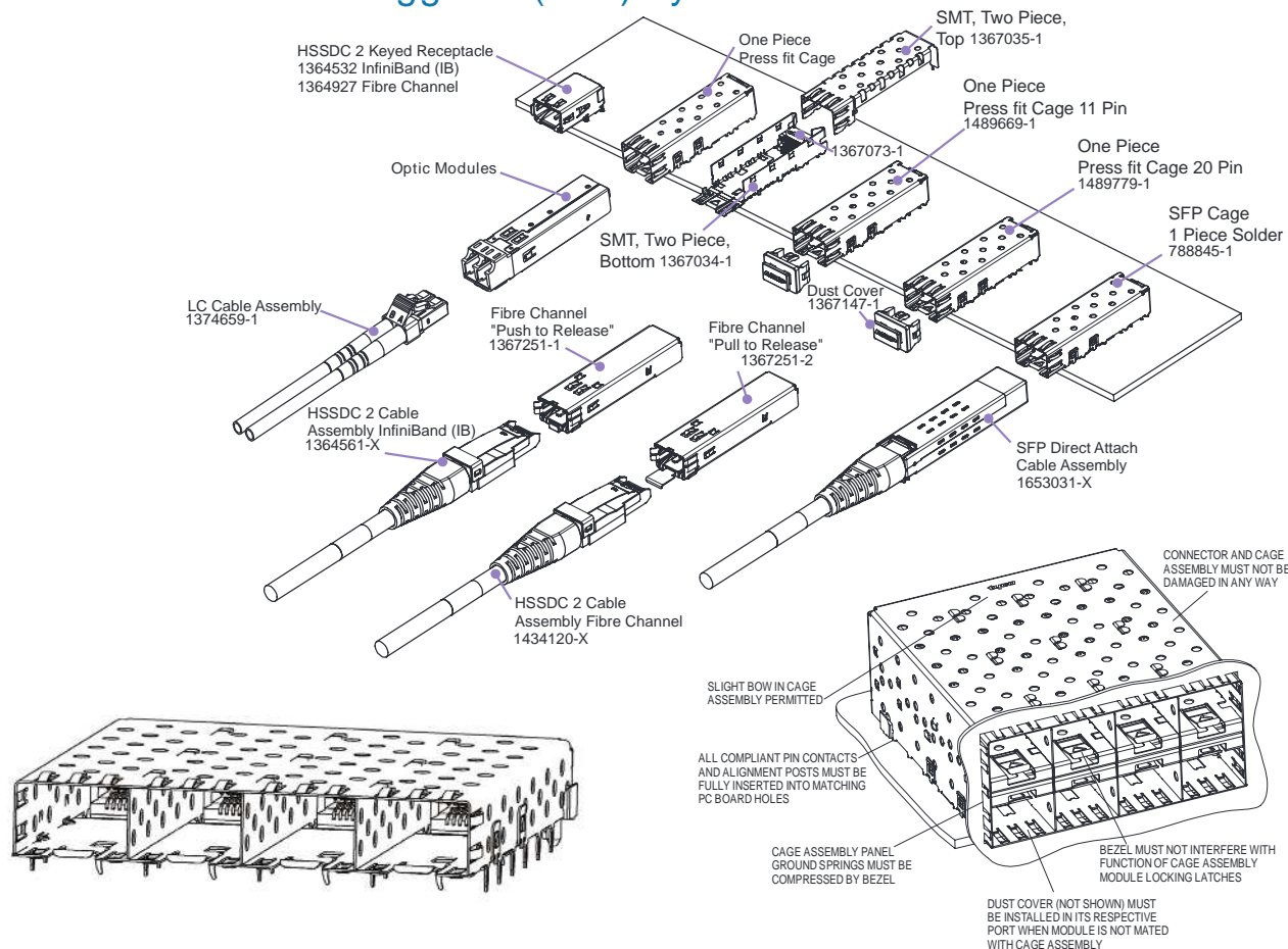
1 x 4 Cage Assembly
