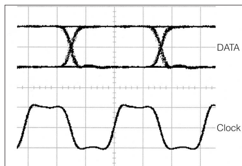
H: 100 ps/div, V: 1 V/div MU163220A output waveform (3.2 GHz)
