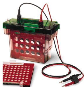
The Criterion blotter as assembled with wire electrodes (#170-4071)
