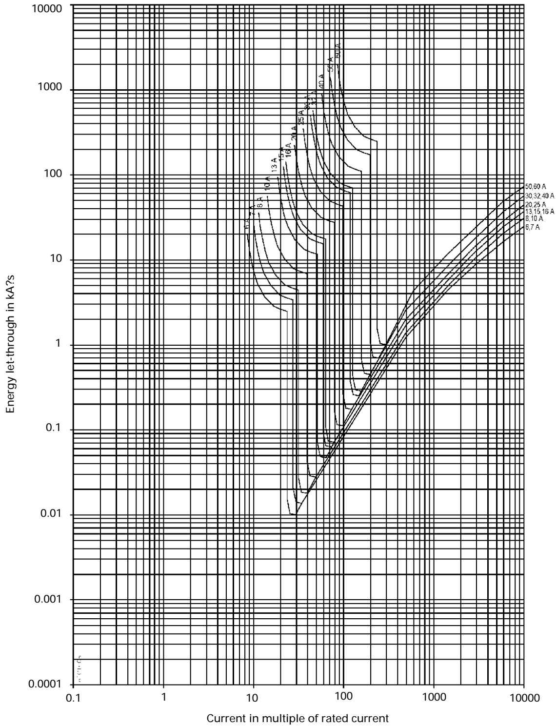
MCB TYPE WMS — CURVE B ENERGY LET-THROUGH CHARACTERISTICS AT 240/415V
