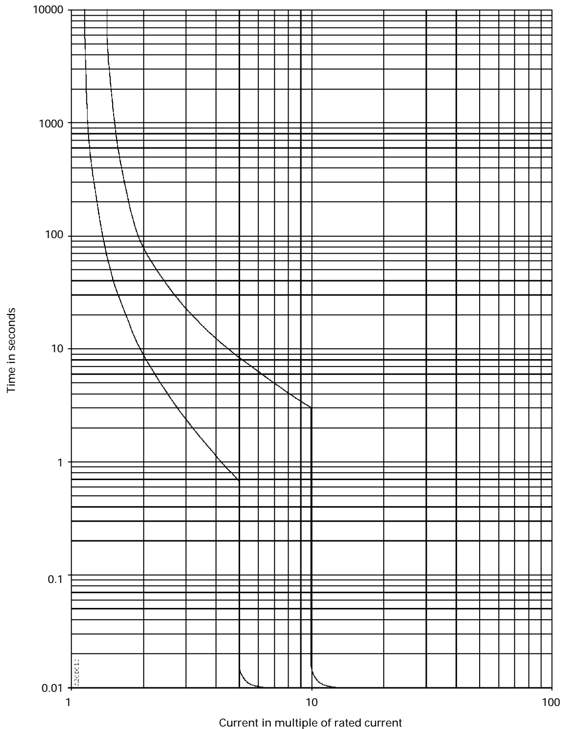
MCB CURVE C TIME-CURRENT CHARACTERISTIC
