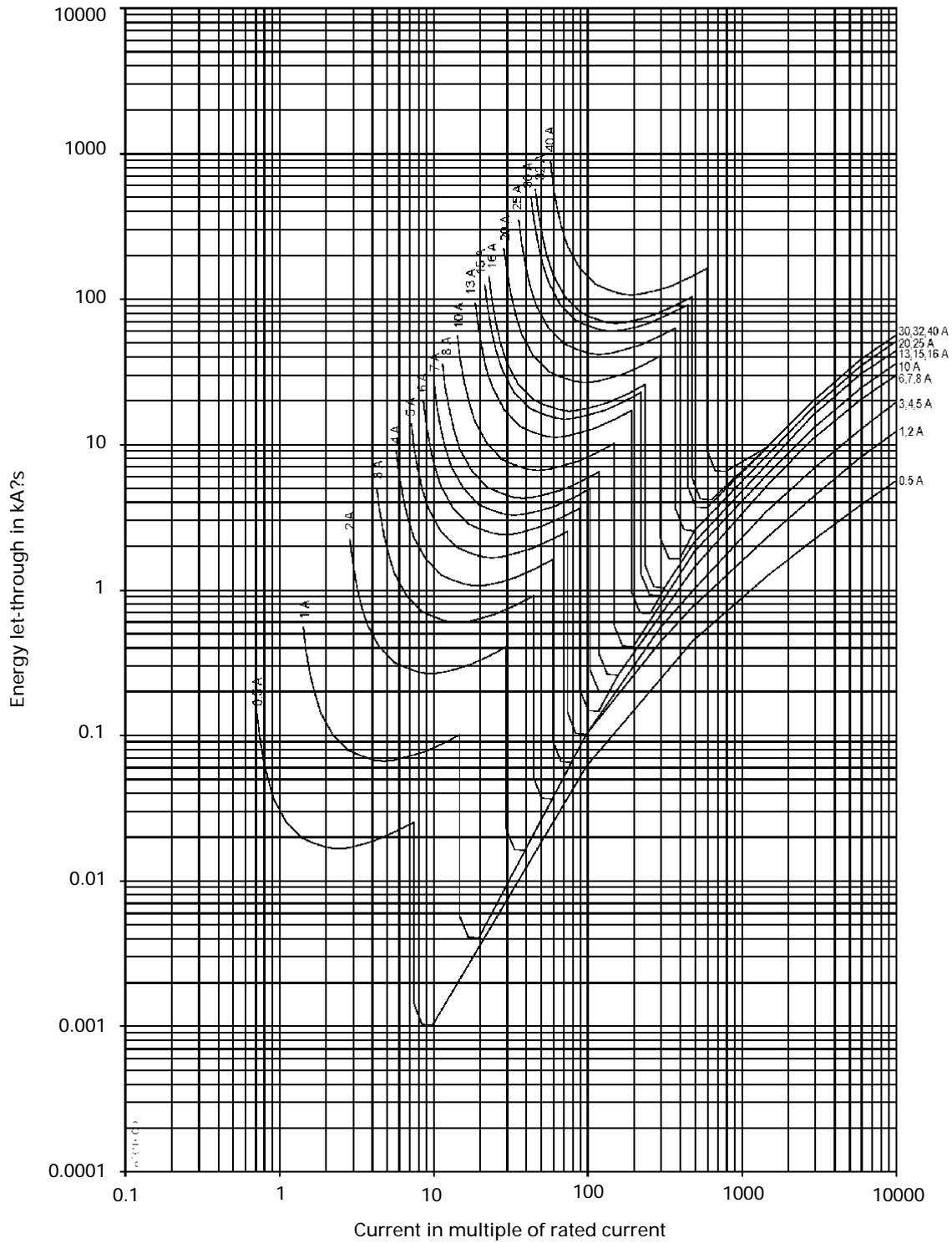
MCB TYPE WMS — CURVE D ENERGY LET-THROUGH CHARACTERISTICS AT 240/415V
