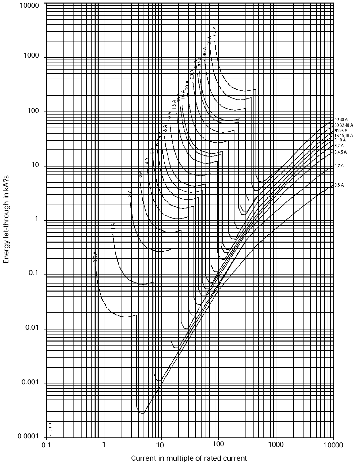
MCB TYPE WMS — CURVE C ENERGY LET-THROUGH CHARACTERISTICS AT 240/415V
