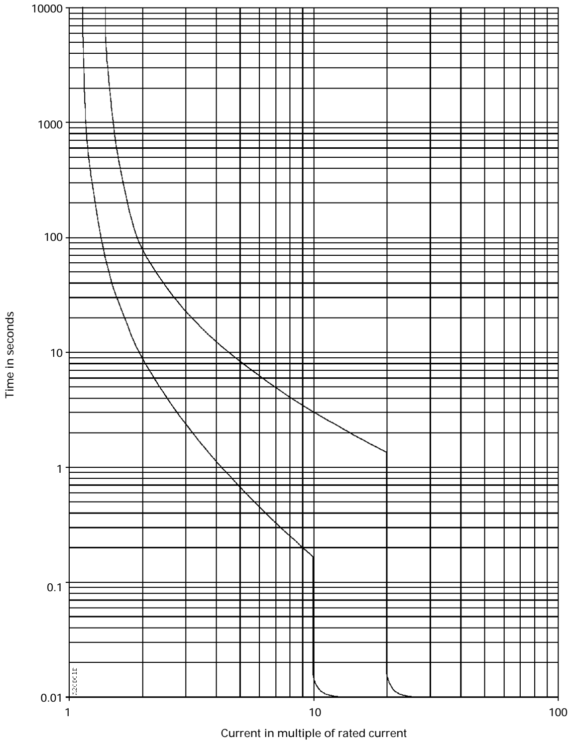
MCB CURVE D TIME-CURRENT CHARACTERISTIC
