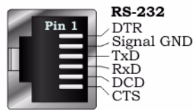
RJ11 Jack (Receptacle) Signals
