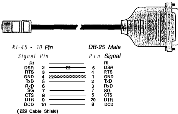
Figure 9 RJ-45 to DB-25 Modem Cable (10 Wire)
