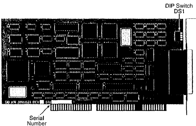
PC/4e and PC/8e Board Layout
