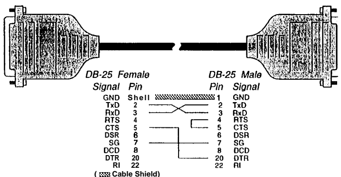
Figure 14 Terminal/Printer Cable with DTR Handshaking (DB-25)
