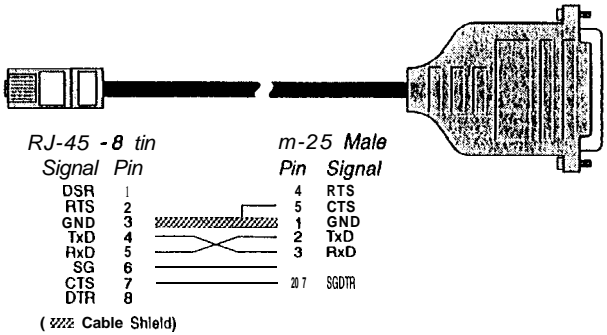
Figure 16 Terminal/Printer Cable with DTA Handshaking (RJ-45)
