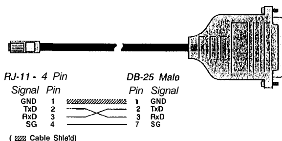
Figure 15 Simple Terminal/Printer Cable (RJ-45)
