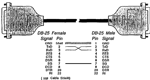
Figure 13 Simple Terminal/Printer Cable (DB-25)
