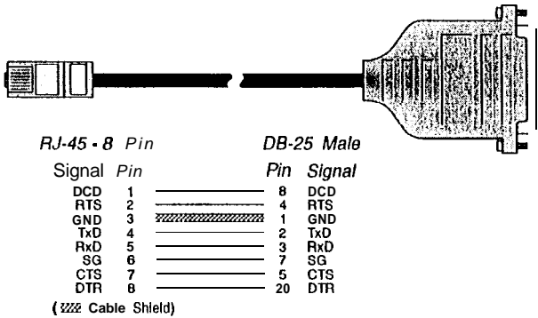
Figure 10 &Wire Modem Cable for use with ALTPIN Configuration
