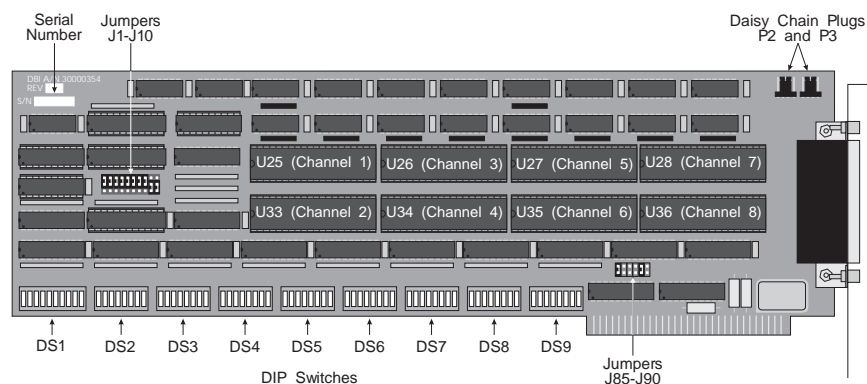
Figure 1 PC/8 Board Layout
