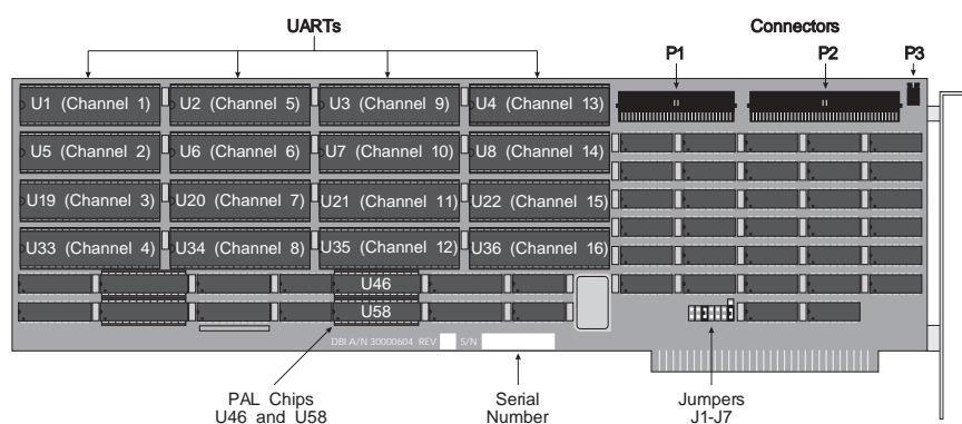
Figure 6 PC/16 Board Layout
