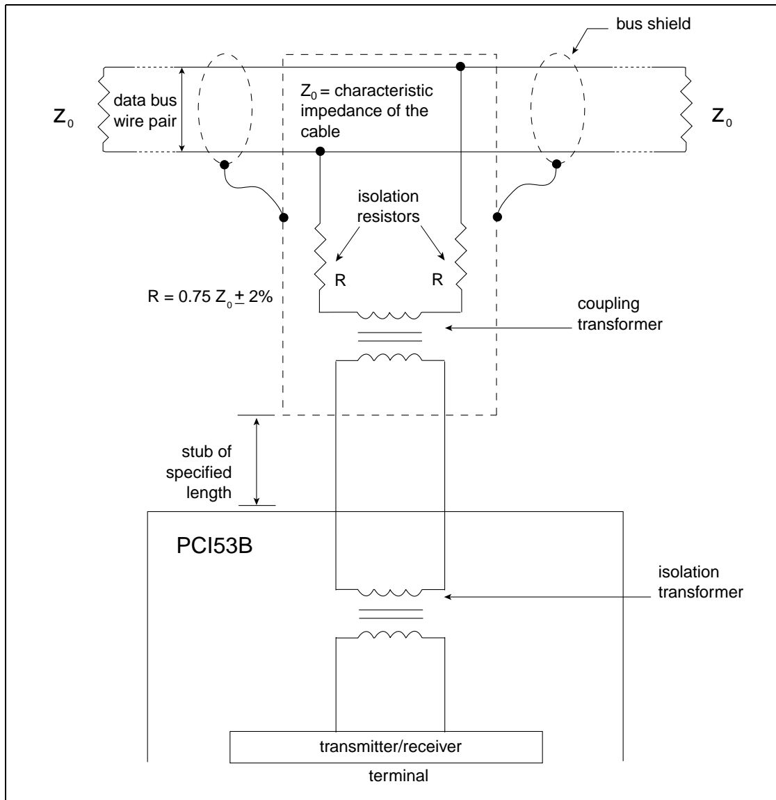
Figure 2. Transformer Coupling
