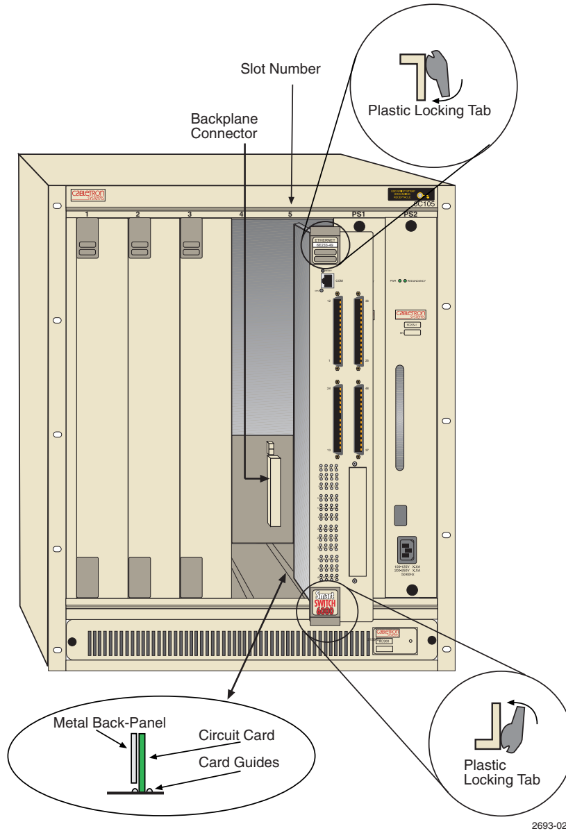
Figure 3-1 Installing an Interface Module
