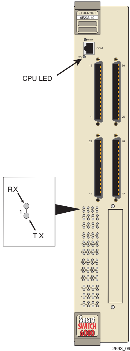
Figure 4-1 LANVIEW LEDs
