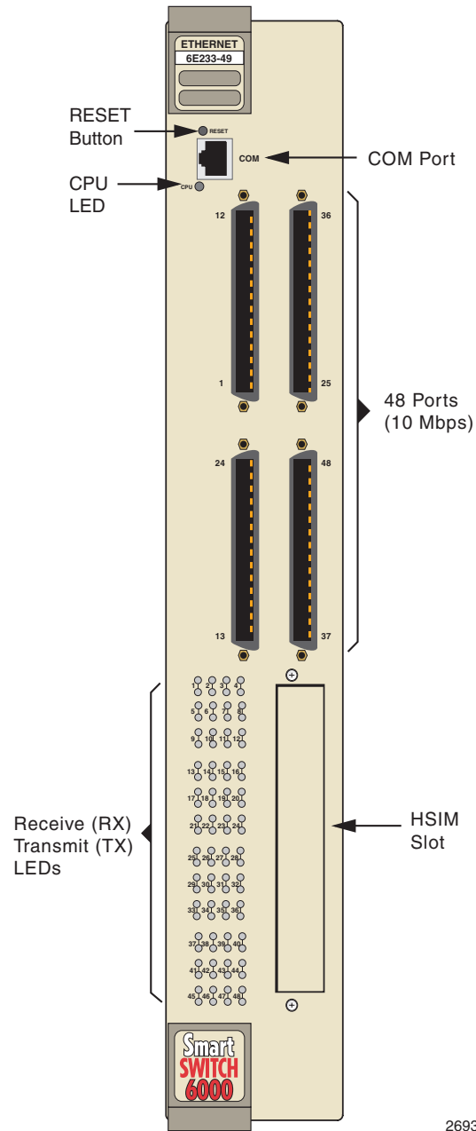
Figure 1-1 The 6E233-49 SmartSwitch
