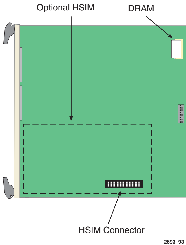
Figure B-4 HSIM Connector Location
