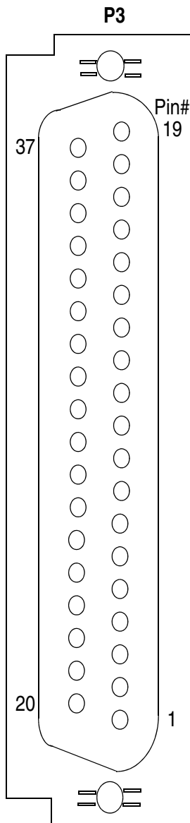
Figure 2-2 P3 Connector
