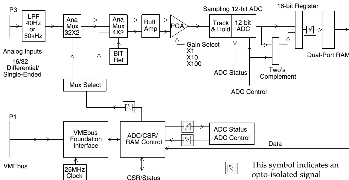
Figure 1-1 VMIVME-3125 Functional Block Diagram
