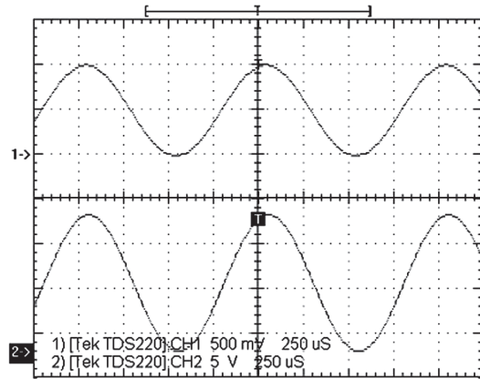
Figure 2. V_{out} = 15\text{ V} , Sine wave, with load
