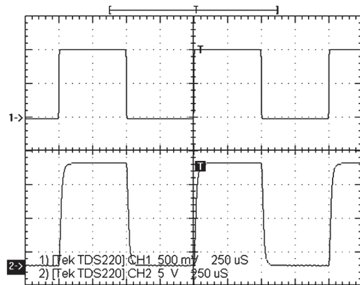
Figure 4. V_{out} = 15\text{ V} , Square wave, with load
