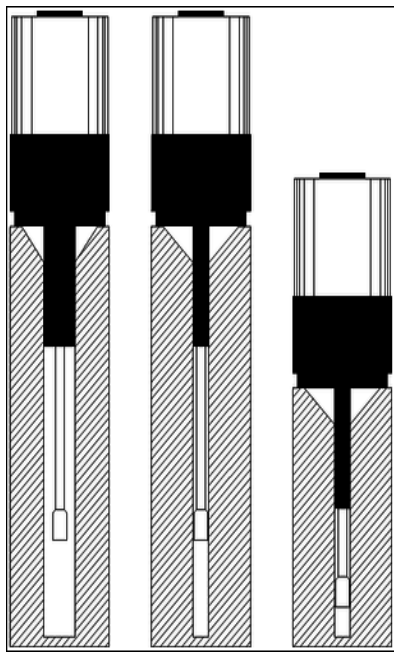
Micro Cuvette Stirring Kit (60MKIT/A)
