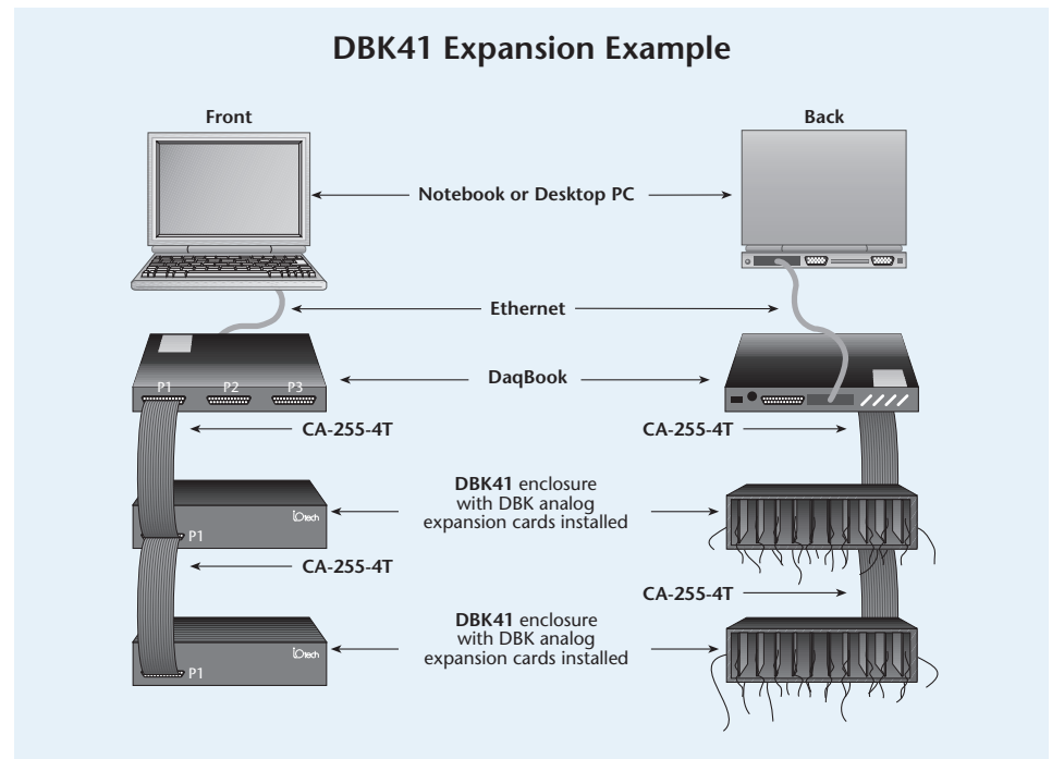
The DBK41 analog expansion module accommodates various analog signal conditioning and expansion cards in one system
