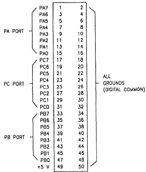
Figure 2-7. 50-pin connector assignments
