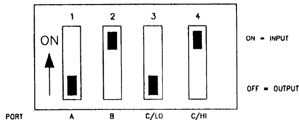
Figure 2-5. Setting the Port Direction Switch
