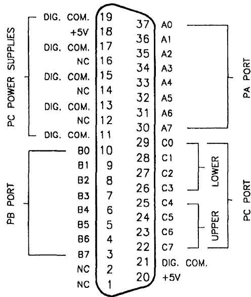
Figure 2-6. 37-pin connector assignments
