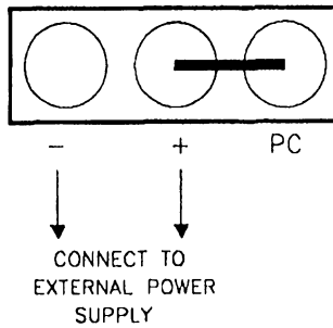
Figure 2-4. Connecting TB7 for external power when the control signals come from a KPCMCIA-PIO24 module.
