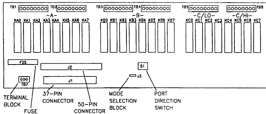
Figure 2-1. Component locations
