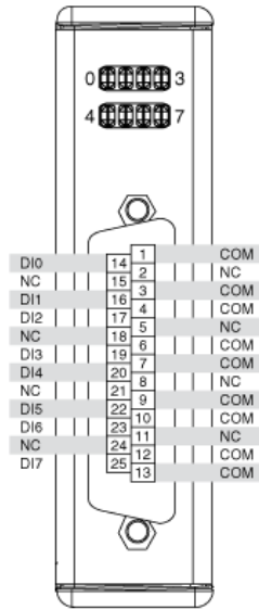
Pin assignments (25-pin)
