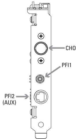
Figure 2. I/O Connector for the PCI-5911
