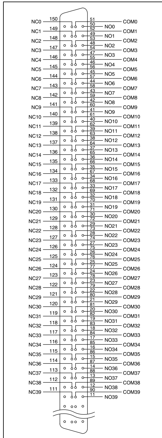
Figure 2. NI PXI-2570 Connector Pinout
