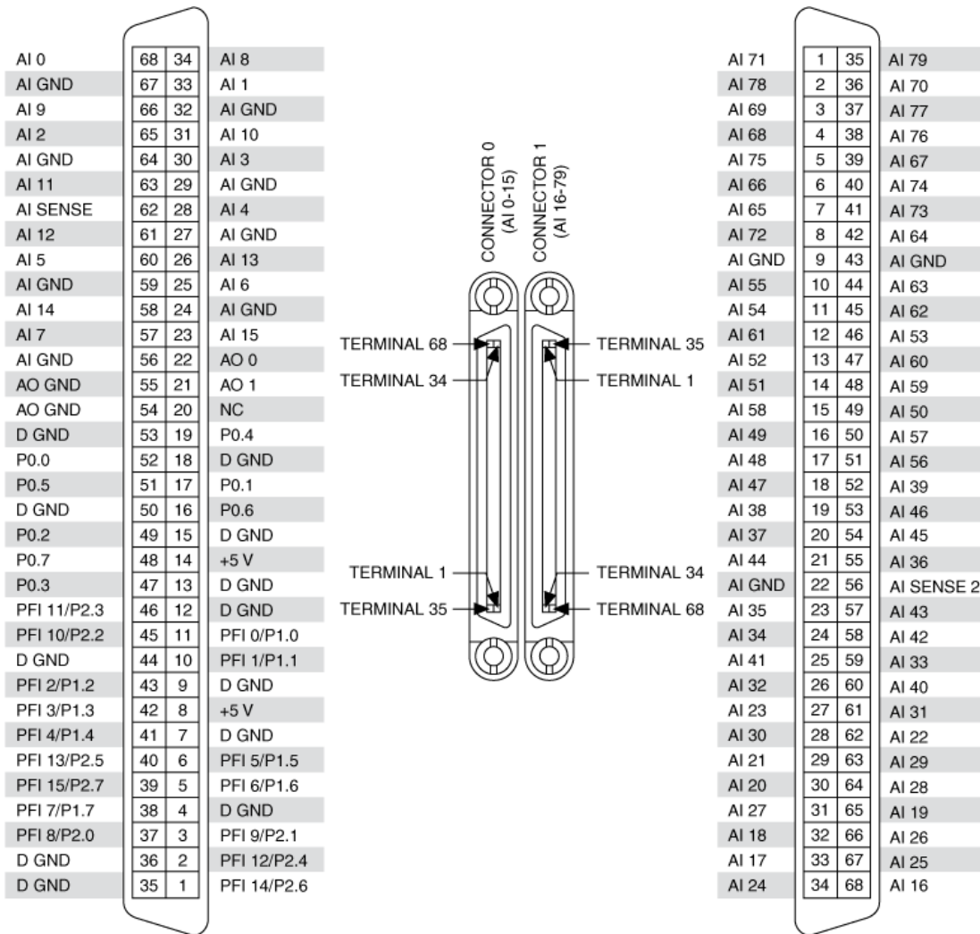
PCI/PXI-6225 Pinout
