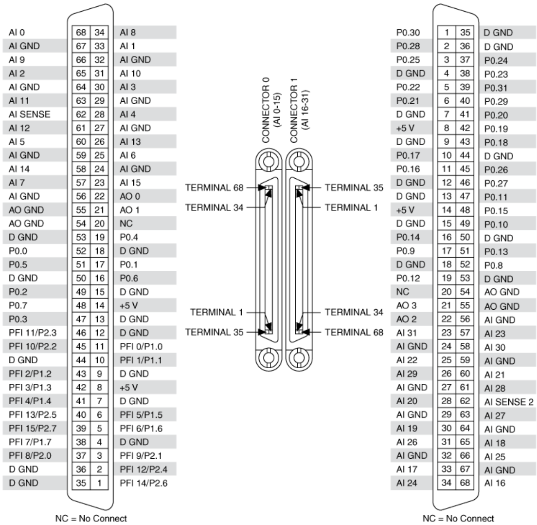
PCI/PXI-6229 Pinout
