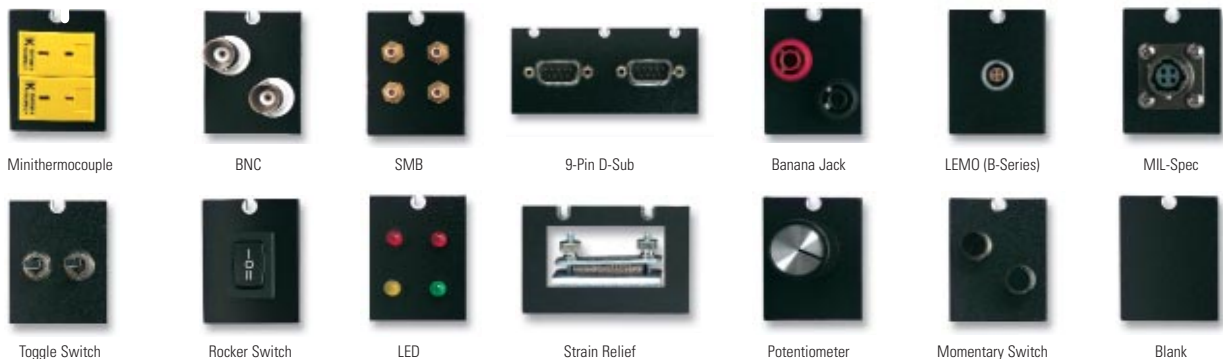
Figure 3. SC-2345 Panelettes Options
