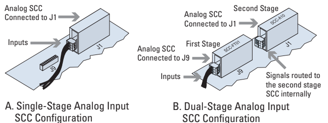
Figure 2. Single-Stage and Dual-Stage Analog Input SCC Configuration for the SC-2345 Connector Block
