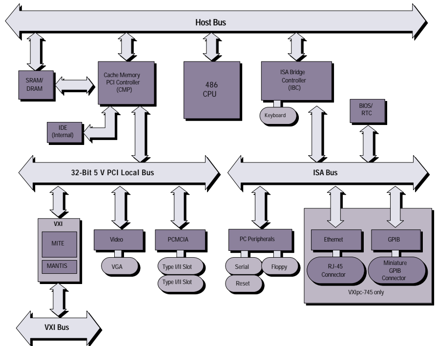
Figure 1. Block Diagram of the VXIpc-700 Series
