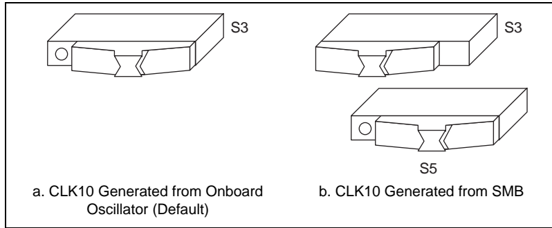
Figure 3-3. VXIbus CLK10 Routing
