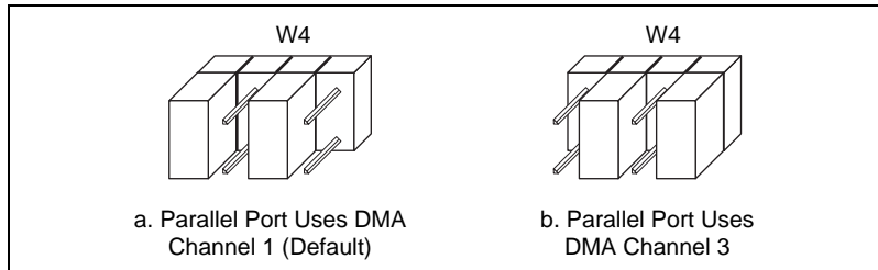
Figure 3-13. Parallel Port DMA Channel
