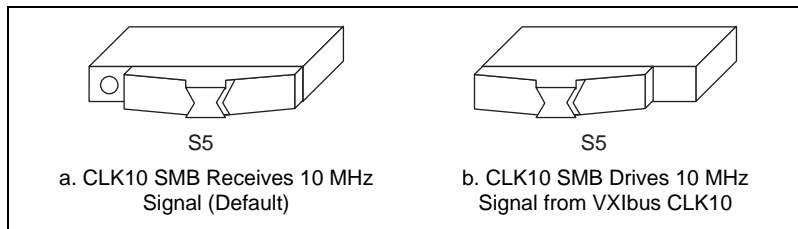
Figure 3-4. SMB CLK10 Direction
