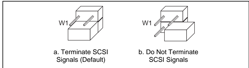
Figure 3-10. SCSI Termination
