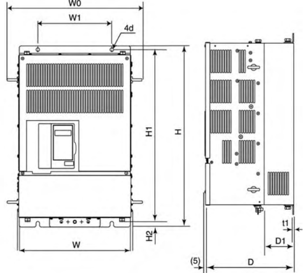
B. 200-V class Inverters of 37 to 110 kW 400-V class Inverters of 75 to 160 kW
