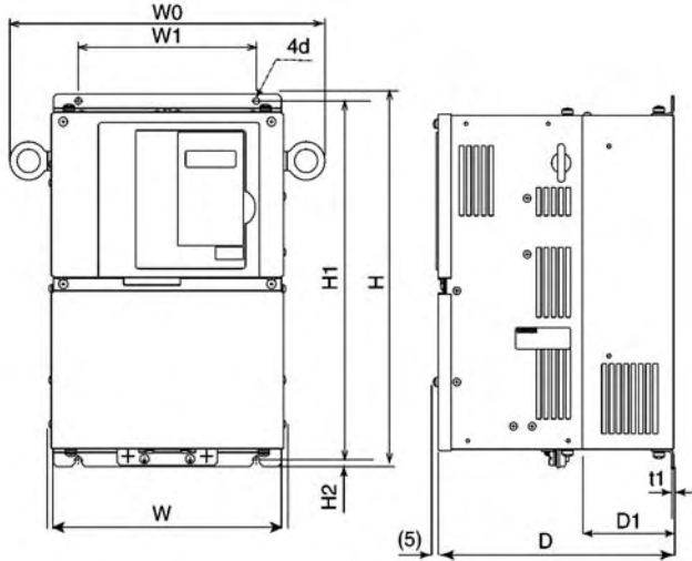
A. 200-V class Inverters of 22 to 30 kW 400-V class Inverters of 22 to 55 kW
