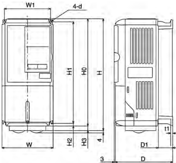
C. 200-V/400-V class Inverters of 0.4 to 18.5 kW
