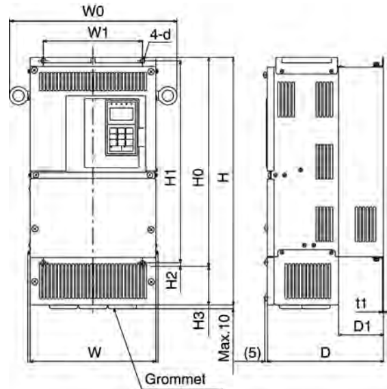
D. 200-V class Inverters of 22 to 75 kW 400-V class Inverters of 22 to 160 kW
