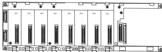
C200H-BC081-V2
