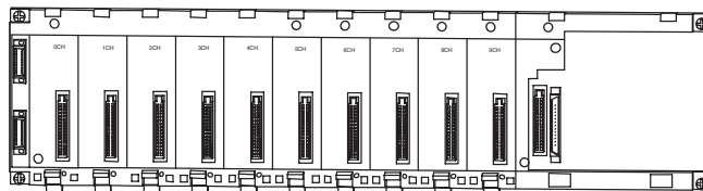
C200H-BC101-V2
