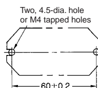
Mounting Holes
