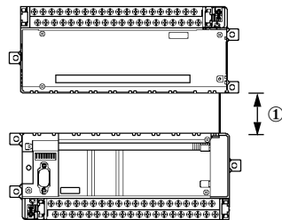
Mounting horizontally
