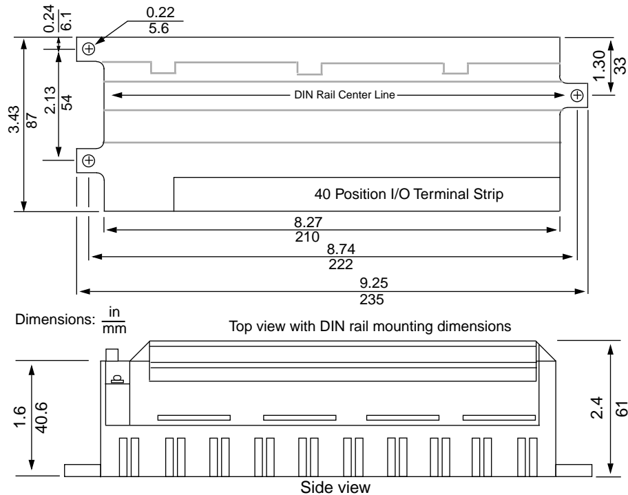
Figure 1: Dimensions
