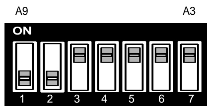
Figure 2 - DIP-switch Illustration
