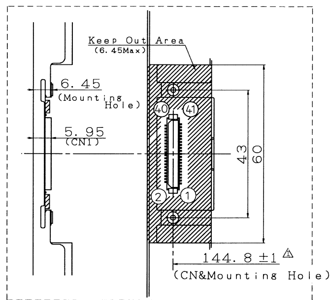
DETAIL A
