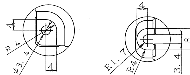
DETAIL G DETAIL H
