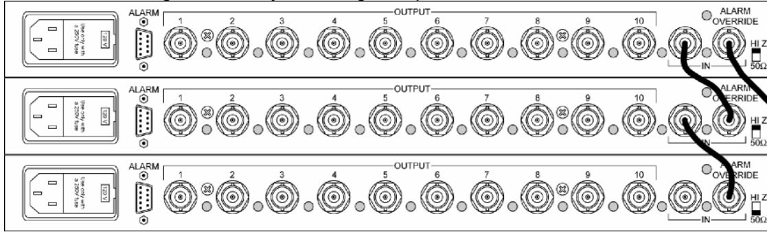
Figure 4. Daisy Chaining Multiple Modules
