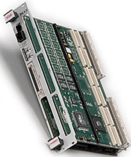
PEX3 CARRIER BOARD PROVIDES THREE PMC SITES
