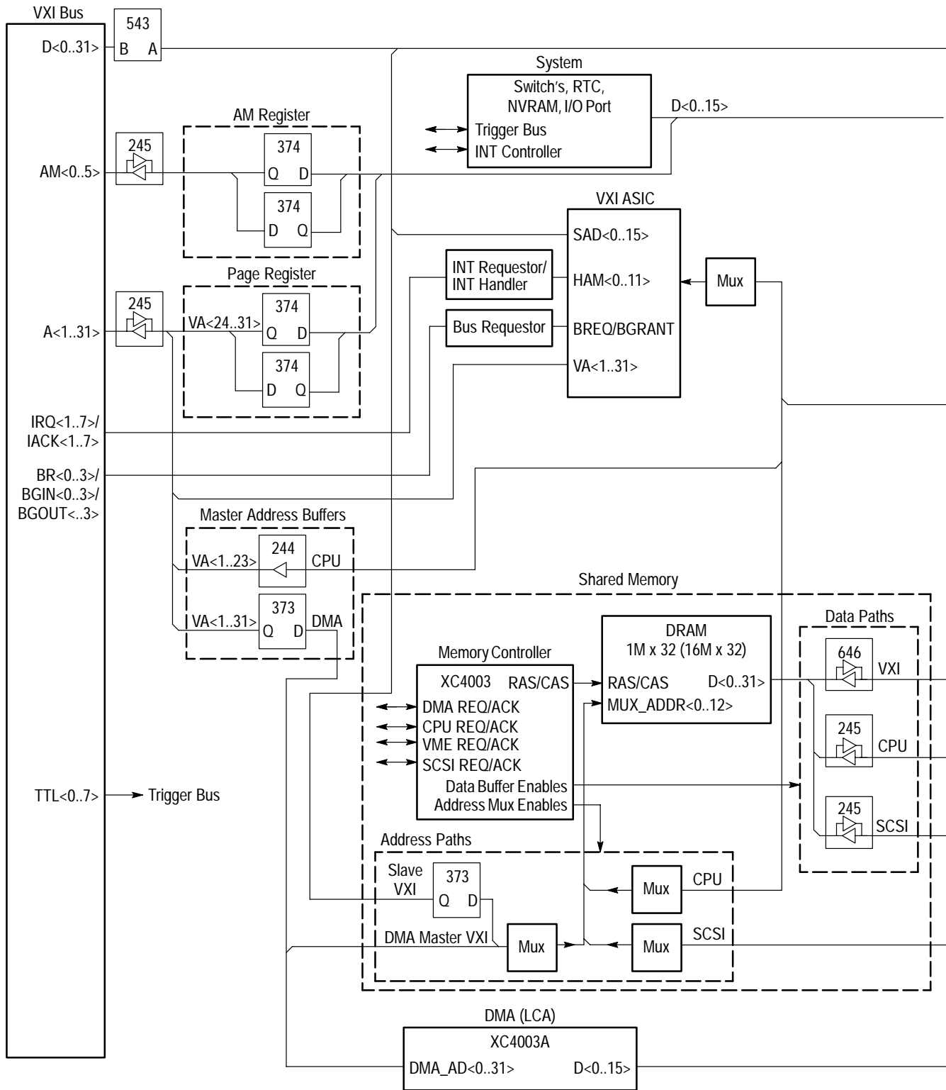
Figure 1-1: VX4570 Block Diagram
