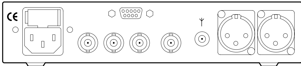
Figure 1-1: Rear panel connectors
