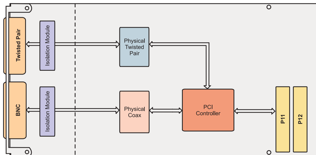
Figure 1-1 : Block Diagram
