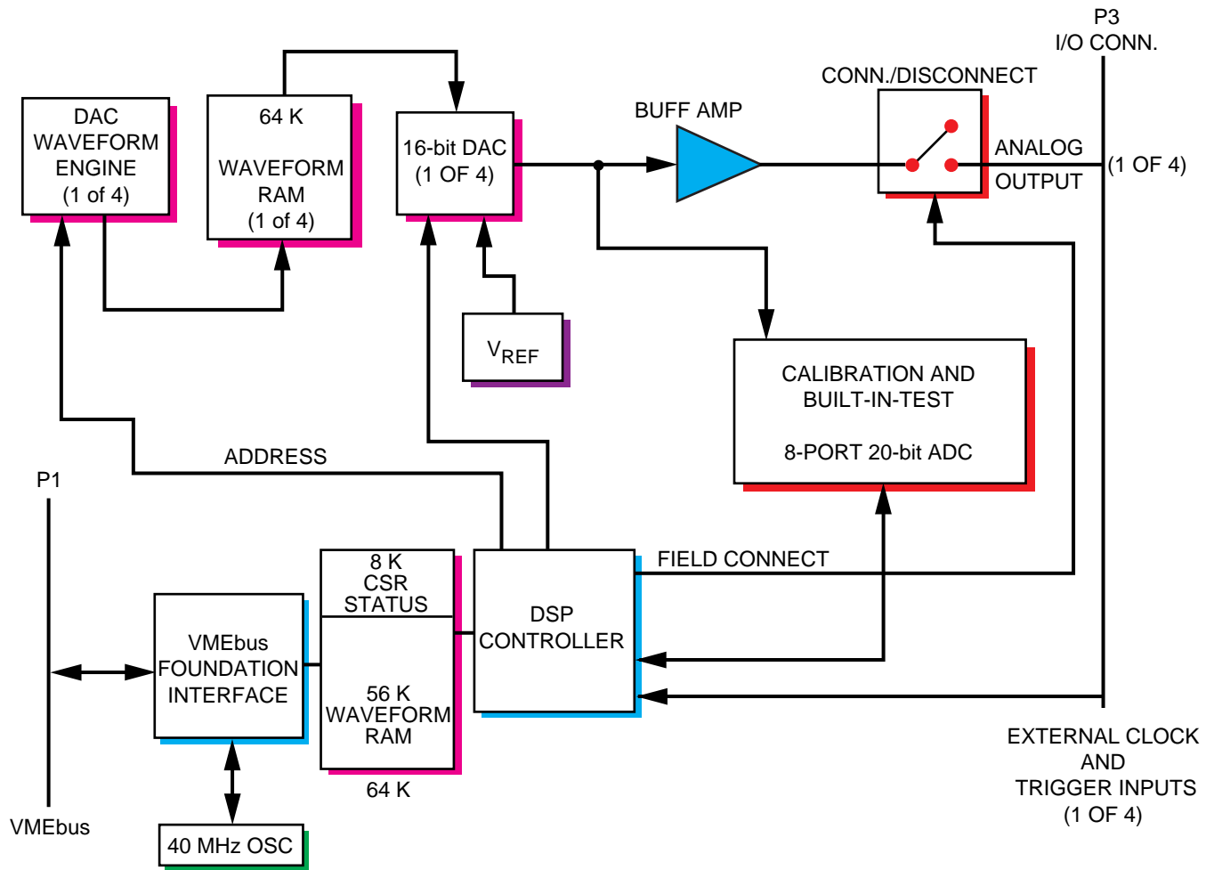
Figure 1. VMIVME-4145 4-Channel Arbitrary Waveform Analog Generator Board with Autocalibration Functional Block Diagram
