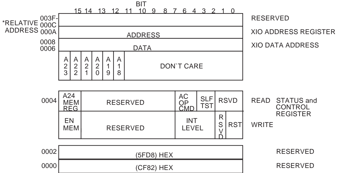
Figure 4.2-1. VMIVME-6000 Configuration Registers
