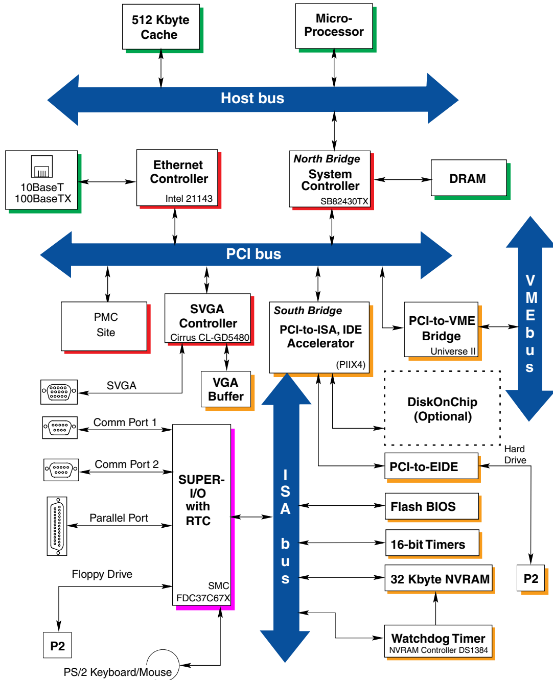
Figure 1. VMIVME-7592 Block Diagram
