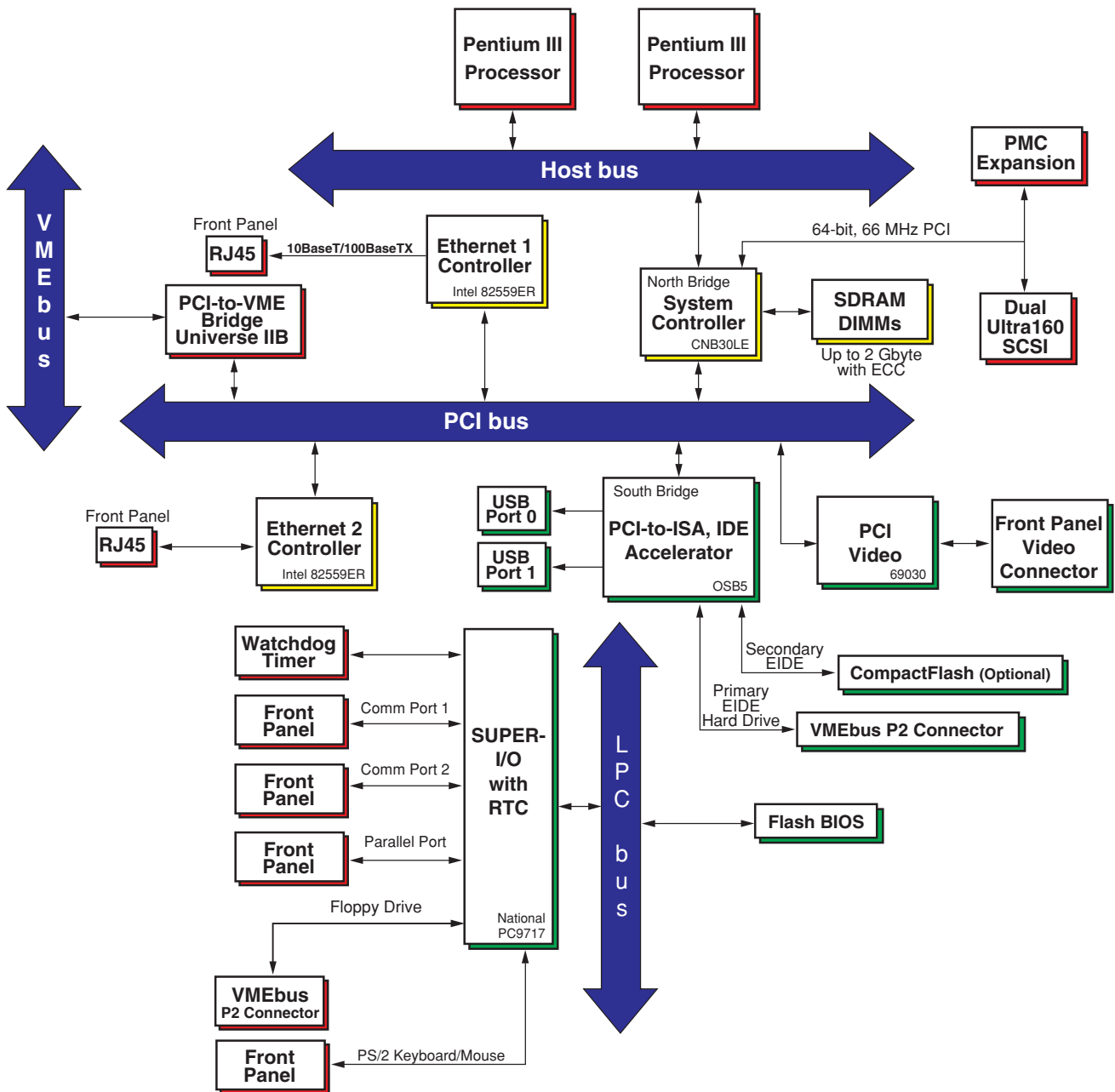
Figure 1. VMIVME-7765 Block Diagram
