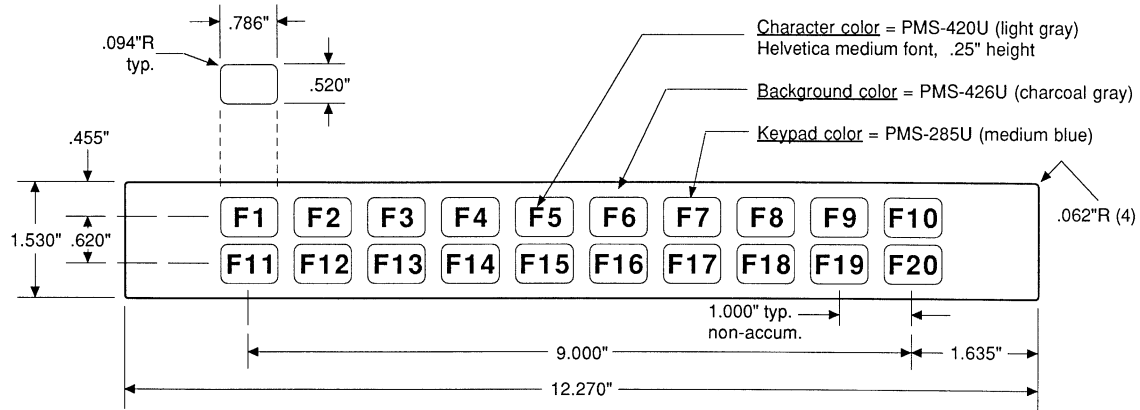
Figure B-3. 9450 Function Key Overlay
